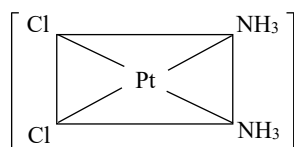
cis-diamminedichlorido platinum(II)
