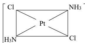
trans- diamminedichlorido platinum(II)
