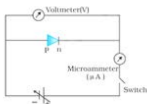
Reverse Bias
