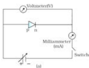
Forward Bias
