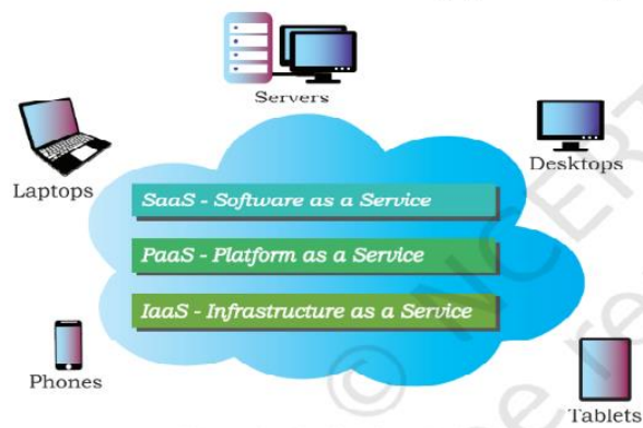
Figure 3.12: Cloud computing
