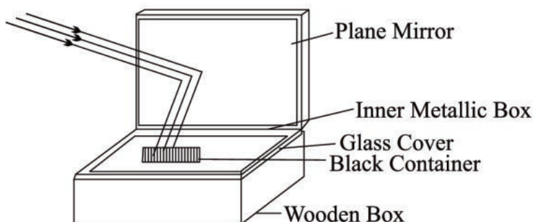
Solar Cooker (Box Type)
