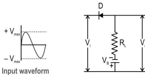
Series negative clipper with negative bias
