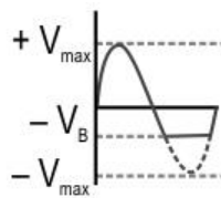
Output waveform
