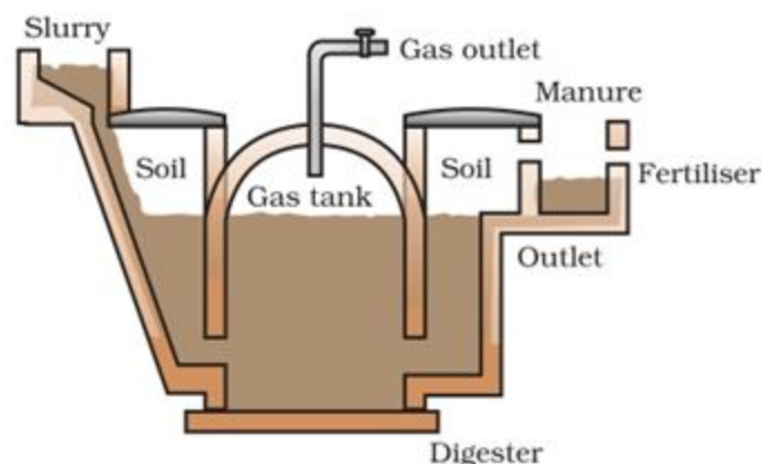
Figure 14.4 Schematic diagram of a bio-gas plant
