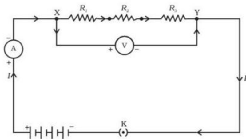
Figure 12.6 Resistors in series
