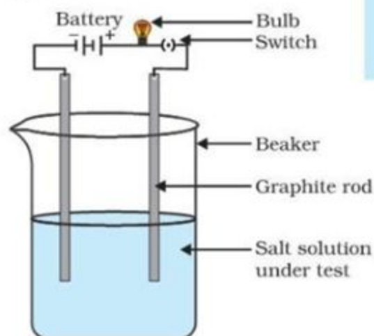
Figure 3.8 Testing the conductivity of a salt solution
