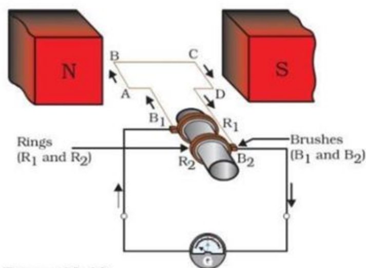
Figure 13.19 Illustration of the principle of electric generator
