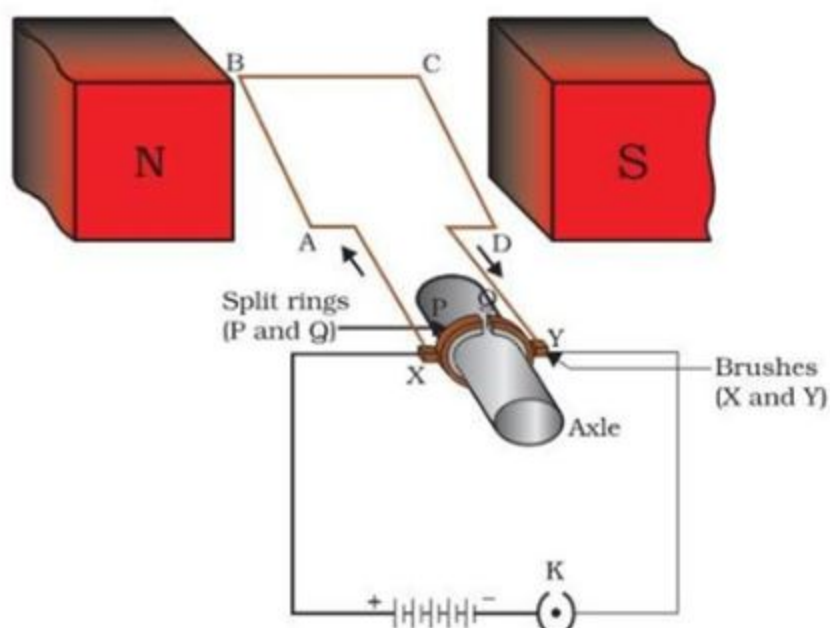
Figure 13.15 A simple electric motor
