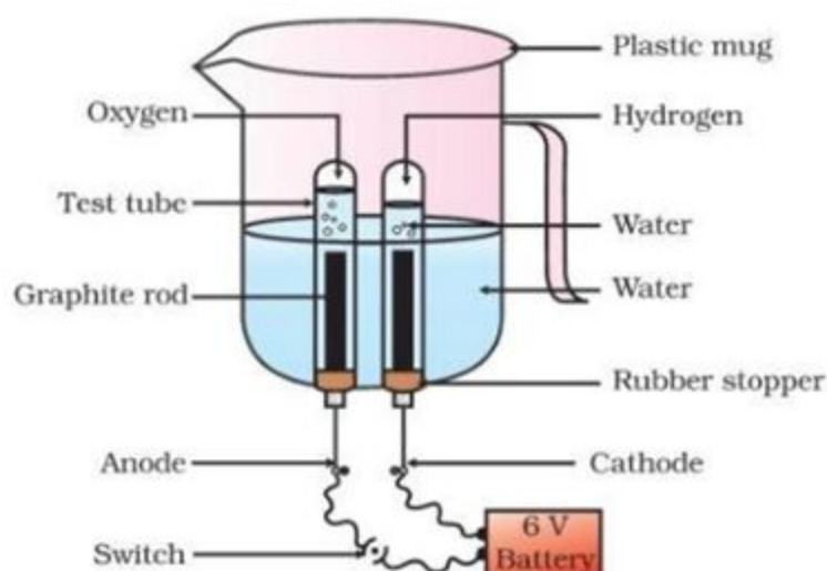
Figure 1.6 Electrolysis of water
