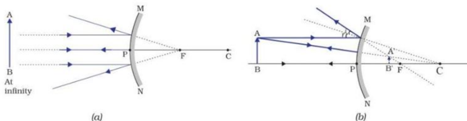
Figure 10.8 Formation of image by a convex mirror
