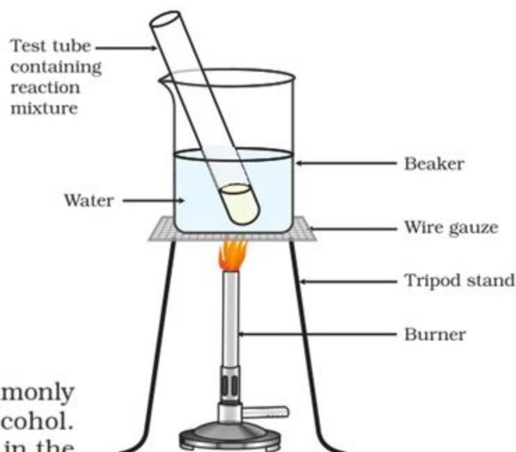
Figure 4.11 Formation of ester
