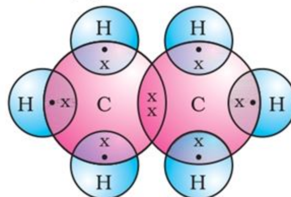
Figure 4.6 (c) Electron dot structure of ethane
