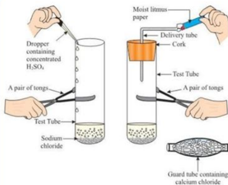
Figure 2.4 Preparation of \text{HCl} gas
