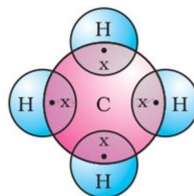
Figure 4.5 Electron dot structure for methane
