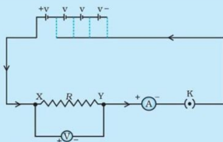
Figure 12.2 Electric circuit for studying Ohm's law
