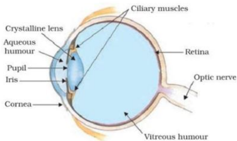
Figure 11.1 The human eye
