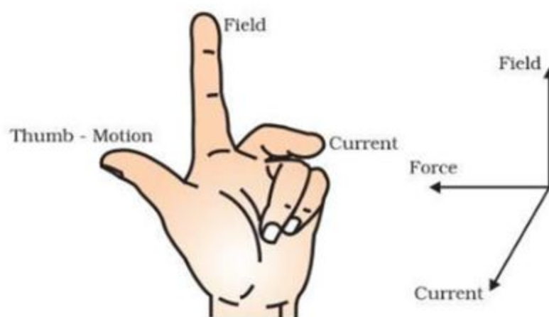
Figure 13.13 Fleming's left-hand rule
