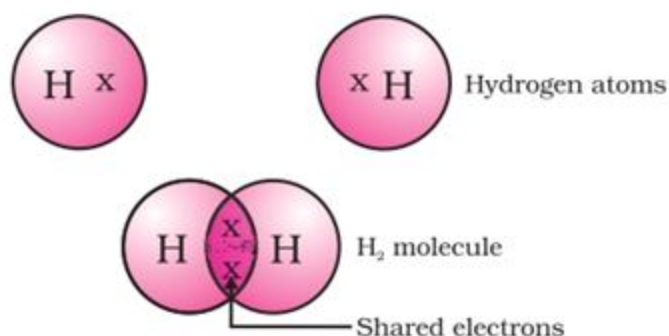
Figure 4.1 A molecule of hydrogen
