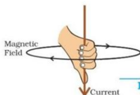
Figure 13.7 Right-hand thumb rule
