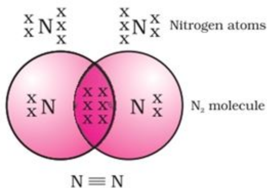
Figure 4.4 Triple bond between two nitrogen atoms
