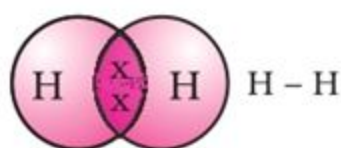
Figure 4.2 Single bond between two hydrogen atoms
