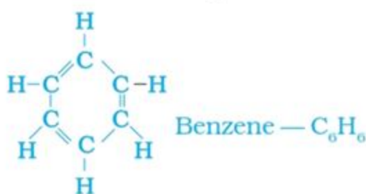
Figure 4.10 Structure of benzene
