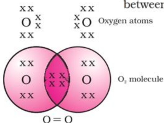
Figure 4.3 Double bond between two oxygen atoms
