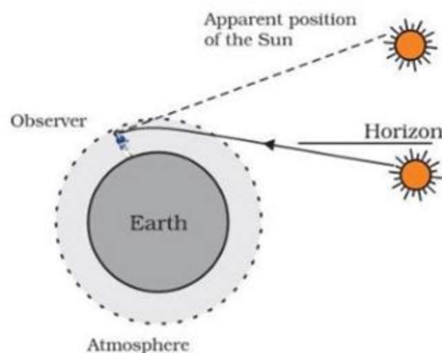
Figure 11.10 Atmospheric refraction effects at sunrise and sunset
