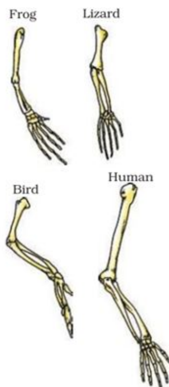
Figure 9.8 Homologous organs
