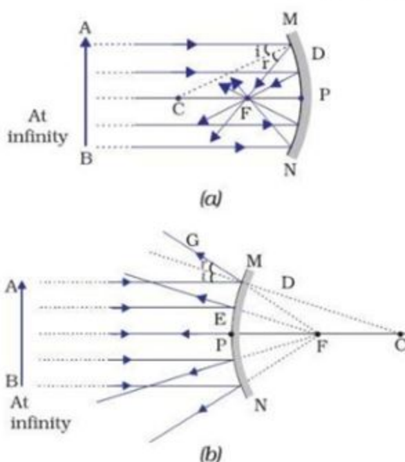
Figure 10.2 (a) Concave mirror (b) Convex mirror
