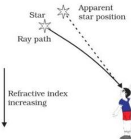
Figure 11.9 Apparent star position due to atmospheric refraction
