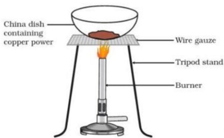
Figure 1.10 Oxidation of copper to copper oxide
