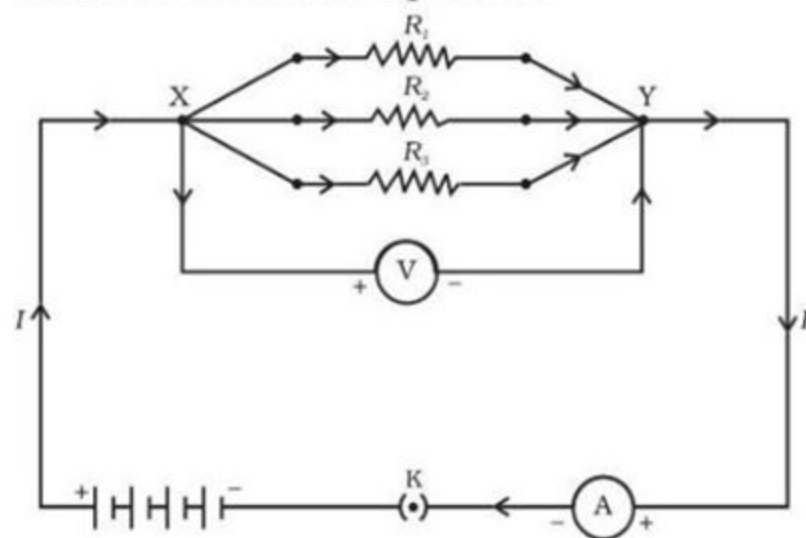
Figure 12.7 Resistors in parallel
