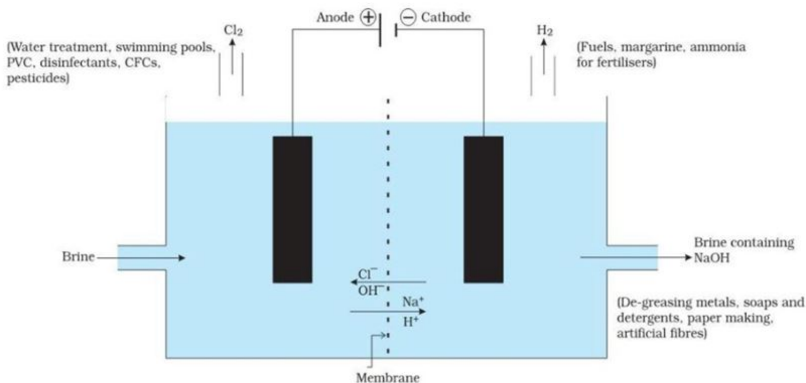
Figure 2.8 Important products from the chlor-alkali process
