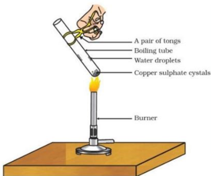
Figure 2.9 Removing water of crystallisation
