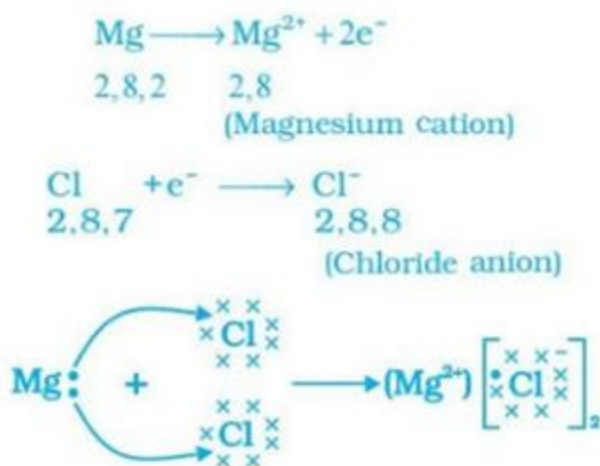
Figure 3.6 Formation of magnesium chloride
