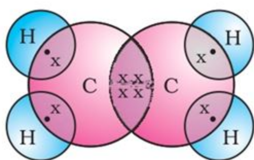
Figure 4.7 Structure of ethene
