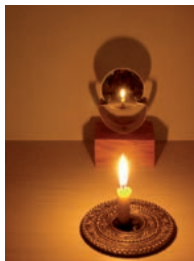
Fig. 11.19 Image formed by a convex mirror
