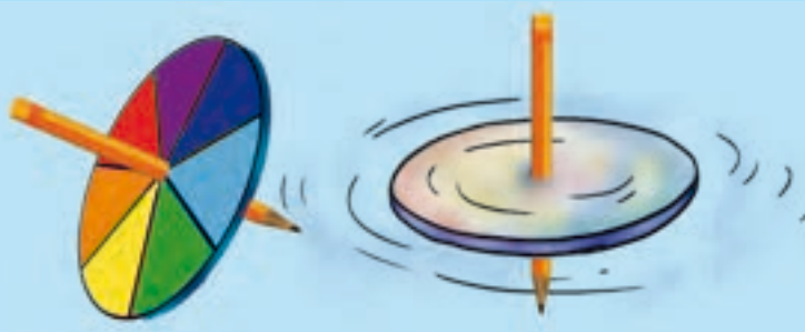
Fig. 11.32 A top with seven colours
