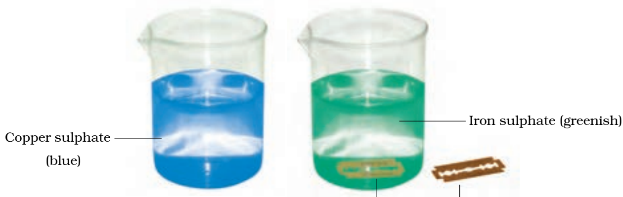
Fig. 5.4 Change in colour of the copper sulphate solution due to reaction with iron
